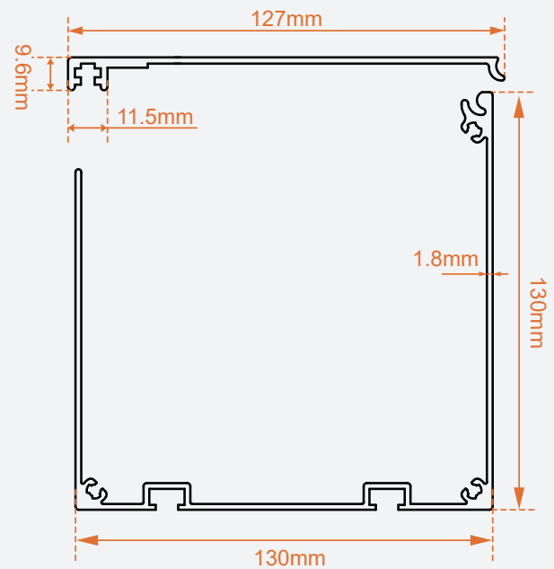
Cassette+Cover
