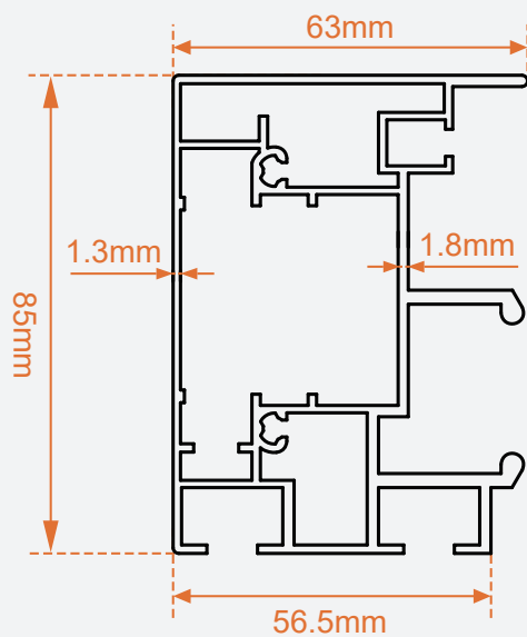
Guide Rail
