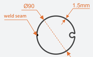
Steel Roller
